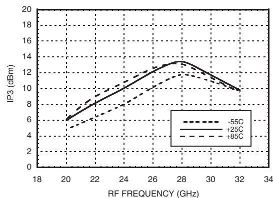
Input P3 vs. Temperature @ LO = -4 dBm, Vdd = +4V
