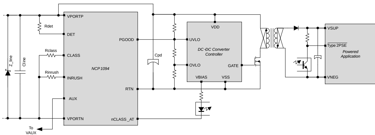
Figure 9. nClass AT indicator / possible implementation with the Powered Device
