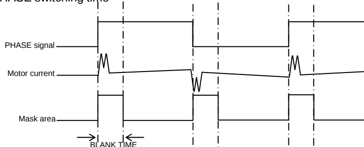
Fig.19 Timing Chart of PHASE Switching Time
