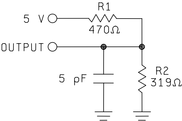
CIRCUIT B OUTPUT LOAD
