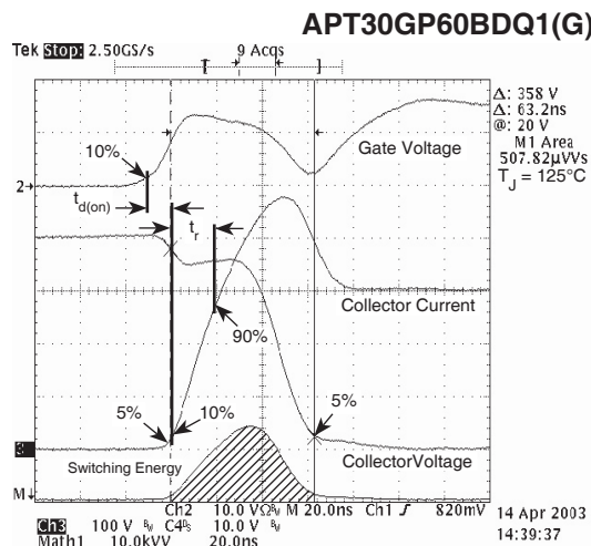
Figure 22, Turn-on Switching Waveforms and Definitions
