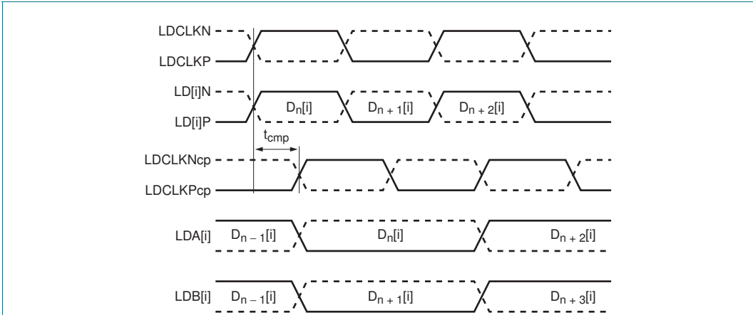
Fig 27. LVDS DDR demux timing (LVDS A and B paths not swapped; LDAB_SWAP = 0)
