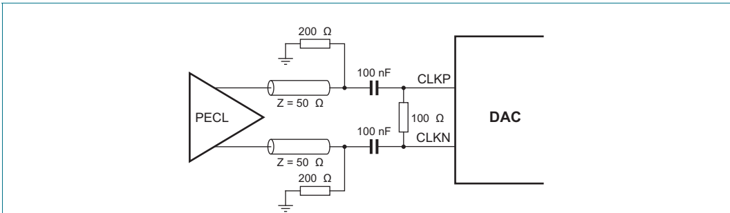
Fig 26. DAC core clock: PECL configuration with AC-coupling
