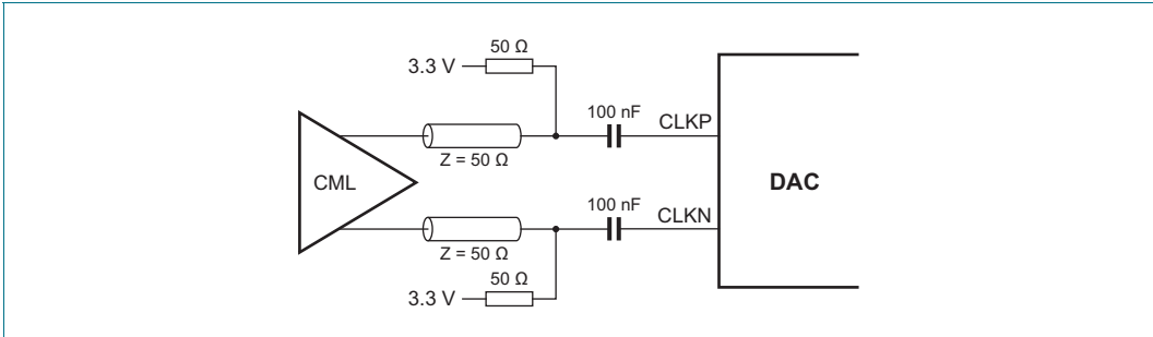
Fig 25. DAC core clock: CML configuration with AC-coupling
