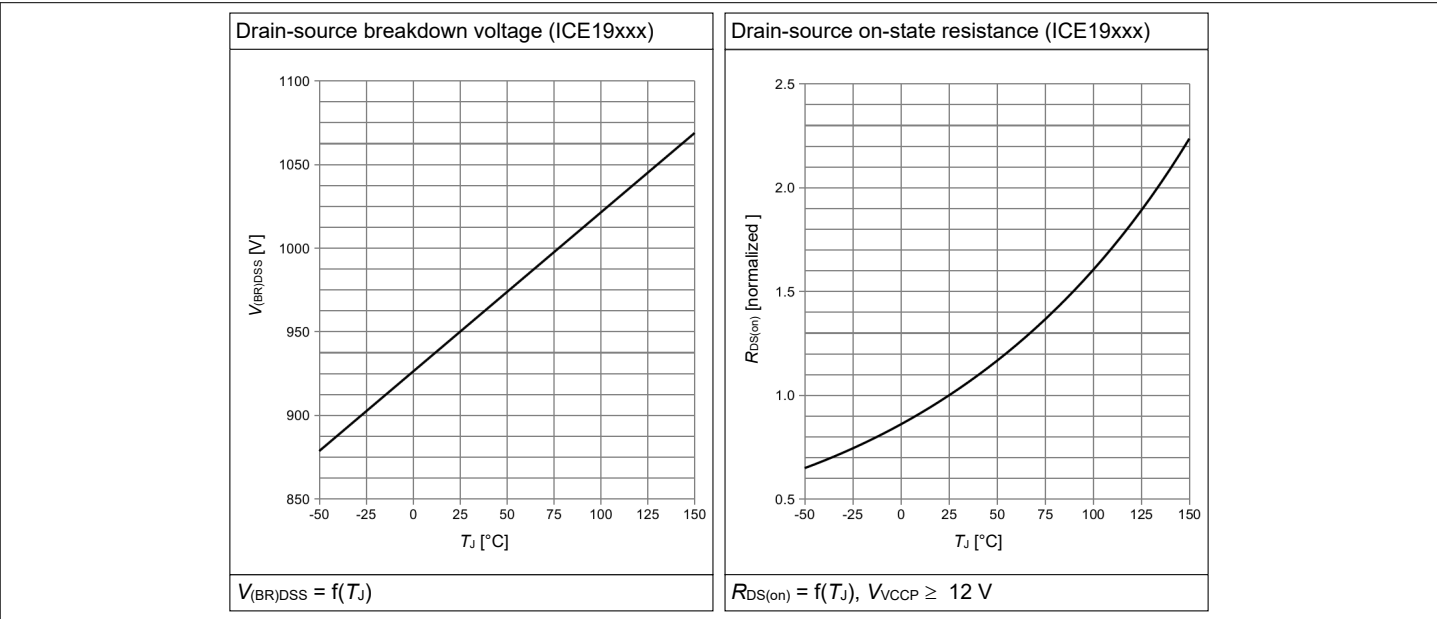
Figure 10 Breakdown voltage and Rds(on) over temperature for ICE19xxx
