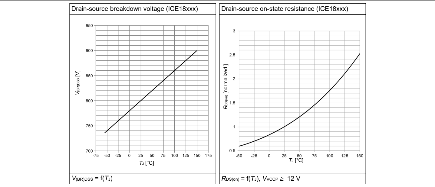
Figure 9 Breakdown voltage and Rds(on) over temperature for ICE18xxx
