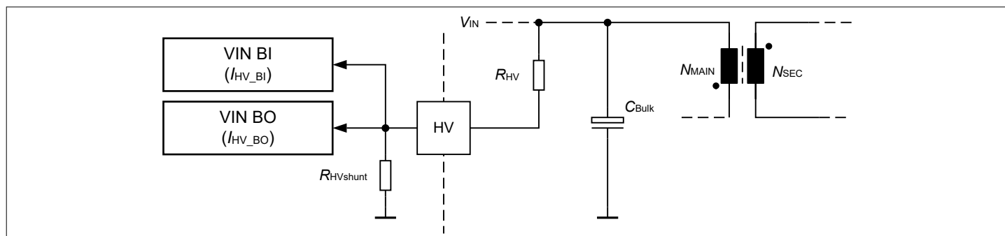
Figure 3 HV pin sensing for brownin/brownout protection
