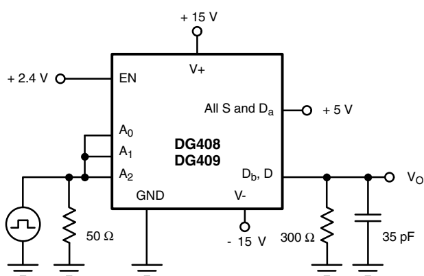
Fig. 4 - Break-Before-Make Interval
