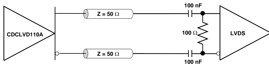
Figure 13. Output AC Termination (With the Receiver Internally Biased)
