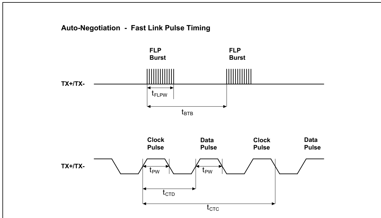
FIGURE 7-15: AUTO-NEGOTIATION TIMING
