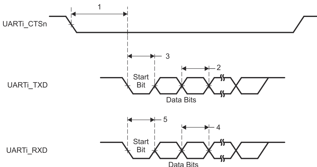
Figure 6-120. UART Timing
