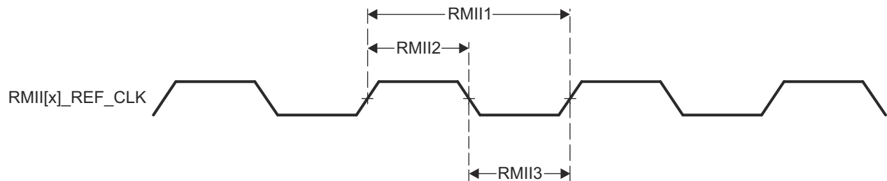
Figure 6-48. RMII[x]_REF_CLK Timing Requirements – RMII Mode
