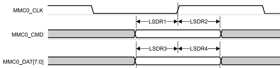
Figure 6-90. MMC0 – Legacy SDR – Receive Mode
