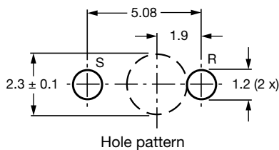
Hole pattern
