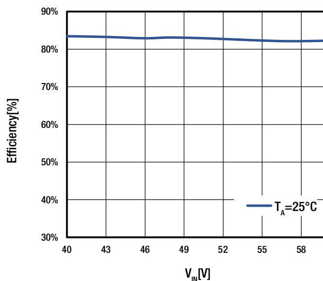
Typical Efficiency vs. Input Voltage
