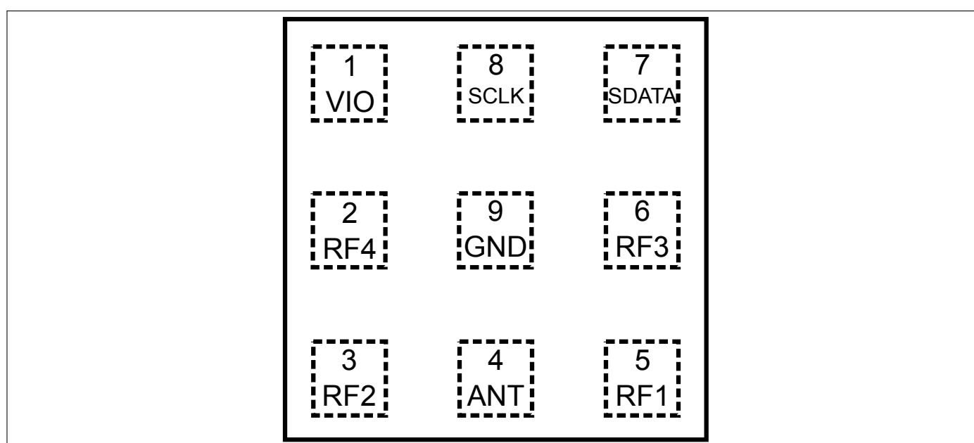
Figure 2: Footprint, top view
