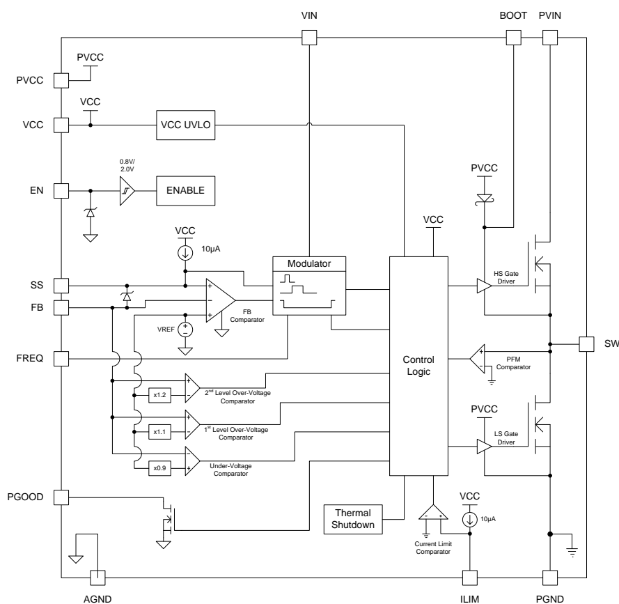
Figure 2. Block Diagram
