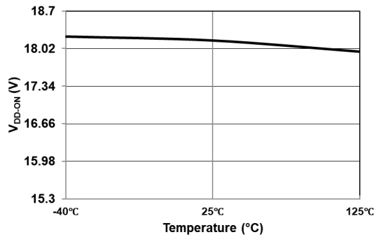
Figure 7. Turn-ON Threshold Voltage ( V_{DD-ON} ) vs. Temperature
