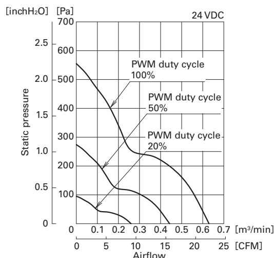
Fig. 11 Airflow vs. static pressure characteristics of 40 × 40 × 28 mm San Ace 40W 9WPA type 24 V, high-speed model
