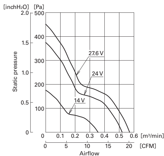
Fig. 13 Airflow vs. static pressure characteristics of 40 × 40 × 28 mm San Ace 40W 9WPA type 24 V, low-speed model
