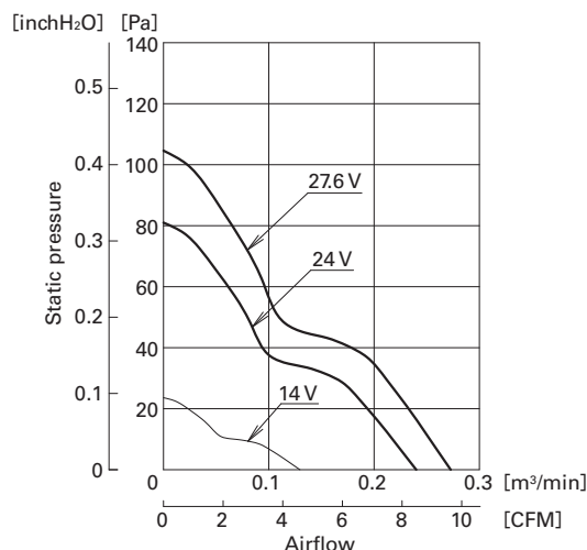
Fig. 9 Airflow vs. static pressure characteristics of 40 × 40 × 20 mm San Ace 40W 9WPA type 24 V, low-speed model
