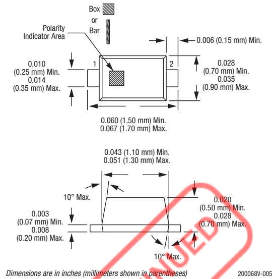
Figure 5. SC-79 Package Dimensions
