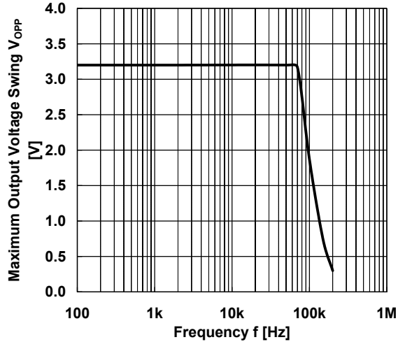
Maximum Output Voltage Swing vs. Frequency V^+=5V, V_{CM}=2.5V, R_L \text{ to } 2.5V, T_a=25^\circ C
