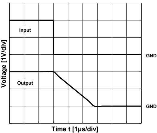
Pulse Response (Fall) V^+=5V, T_a=25^\circ C
