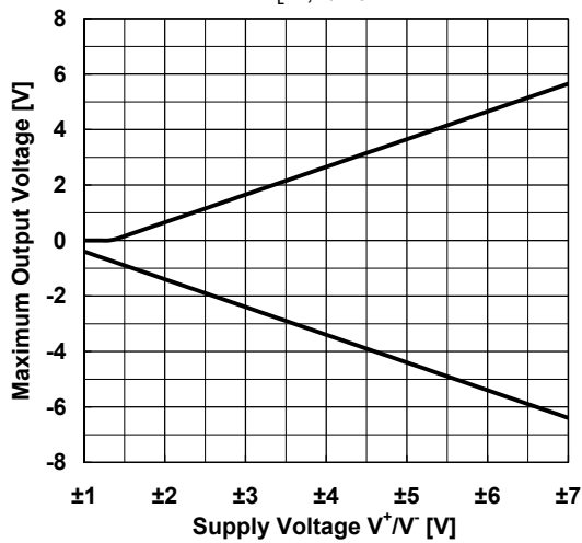
Maximum Output Voltage vs. Supply Voltage R_L = \infty , T_a = 25^\circ\text{C}
