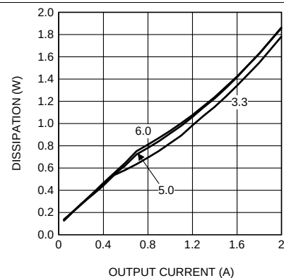
Figure 20. Dissipation 36-V Input, T_A = 85^\circ\text{C}
