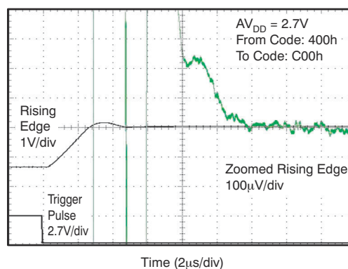
Figure 7-71. Full-Scale Settling Time, 2.7-V Rising Edge
