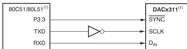
Figure 9-1. DACx311 to 80C51/80I51 Interfaces
