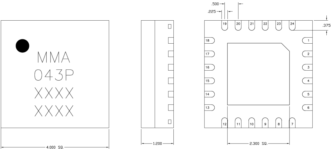
Figure 8 • Package Outline
