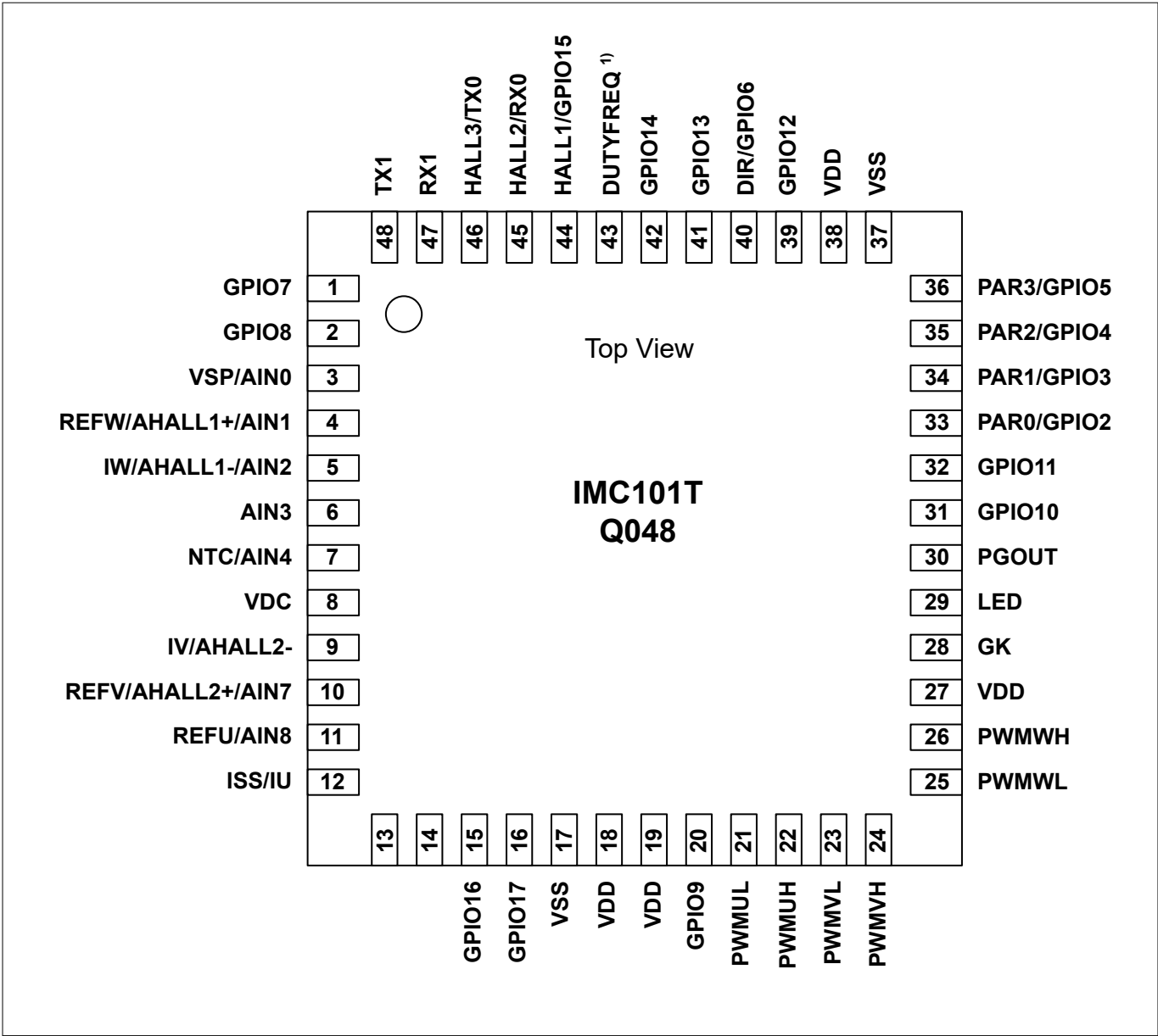
Figure 4 IMC101T-Q048
