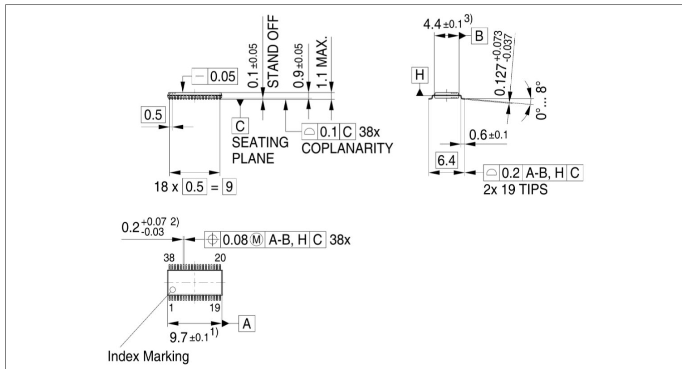
Figure 23 PG-TSSOP-38-9
