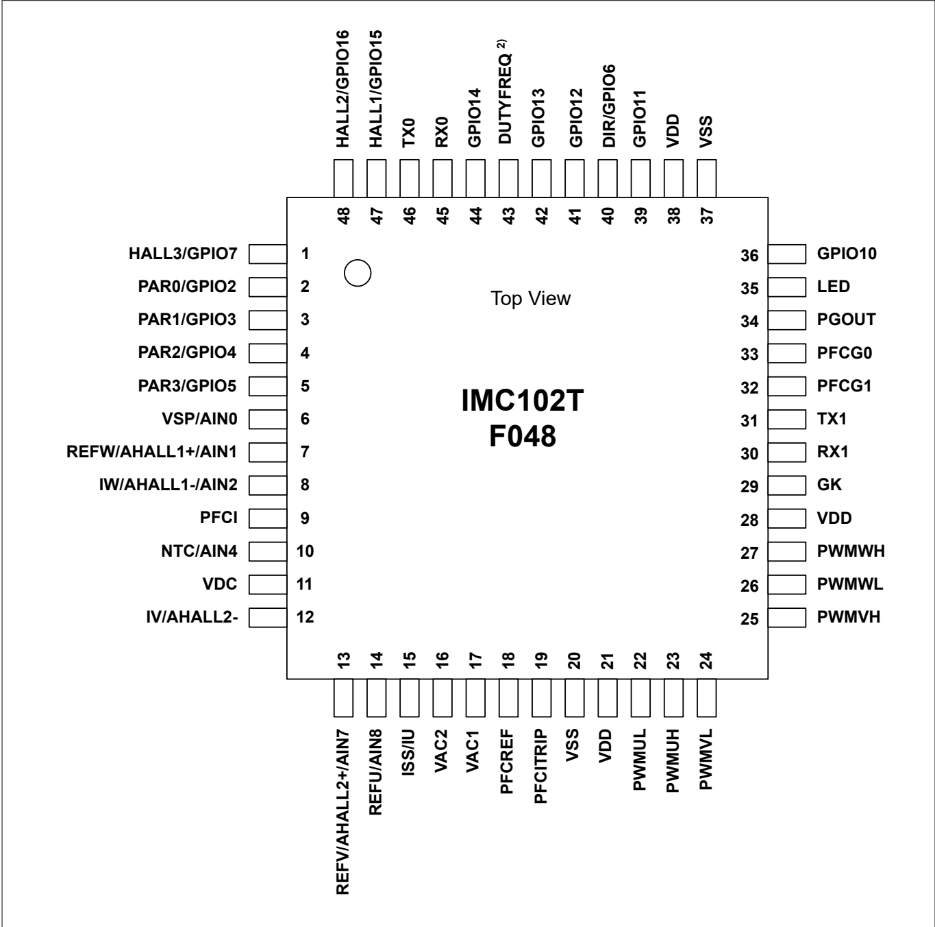
Figure 7 IMC102T-F048
