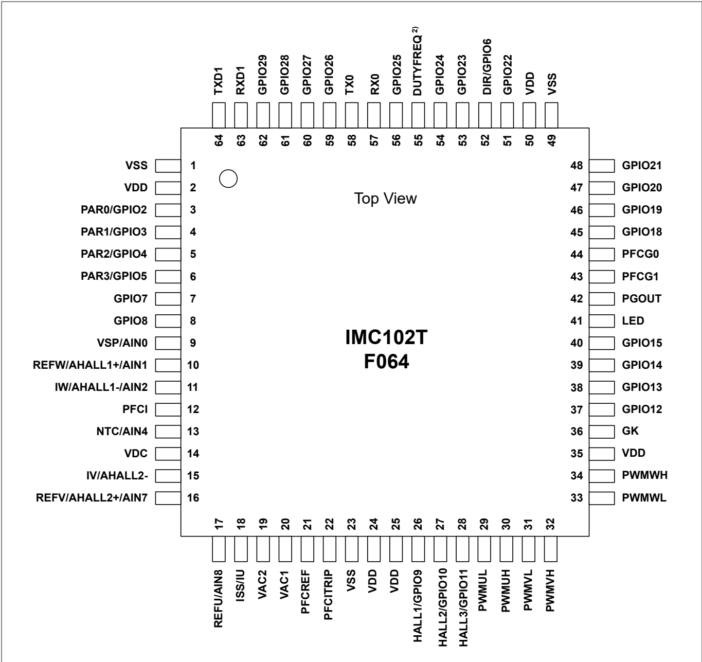
Figure 8 IMC102T-F064
