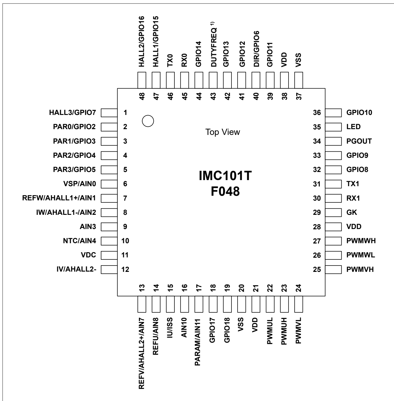
Figure 5 IMC101T-F048
