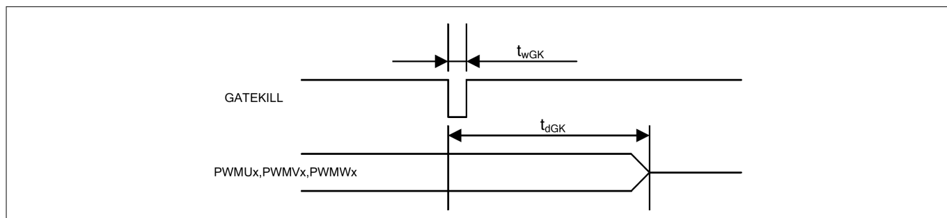
Figure 18 Fault timing
