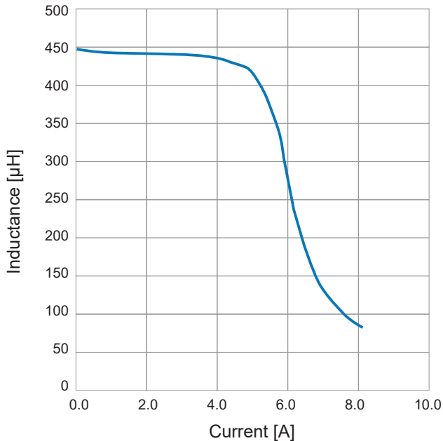
SPFC-RM12-100
