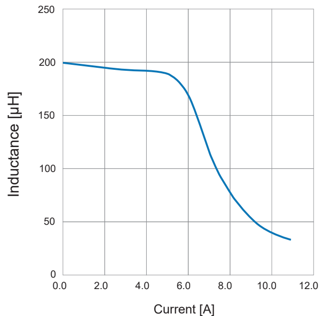
SPFC-EFD30-225
