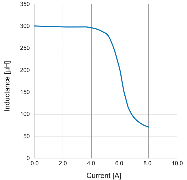
SPFC-PQ38-250
