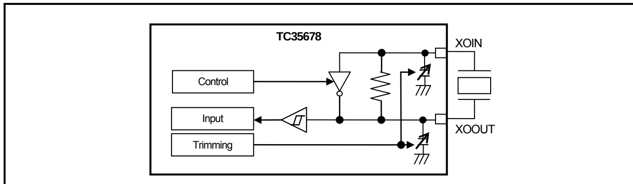
Figure 4-21 Crystal oscillator connection example
