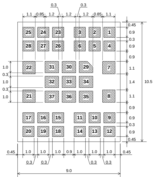
< Bottom View >
