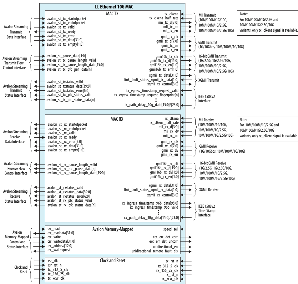
Figure 9. Interface Signals
