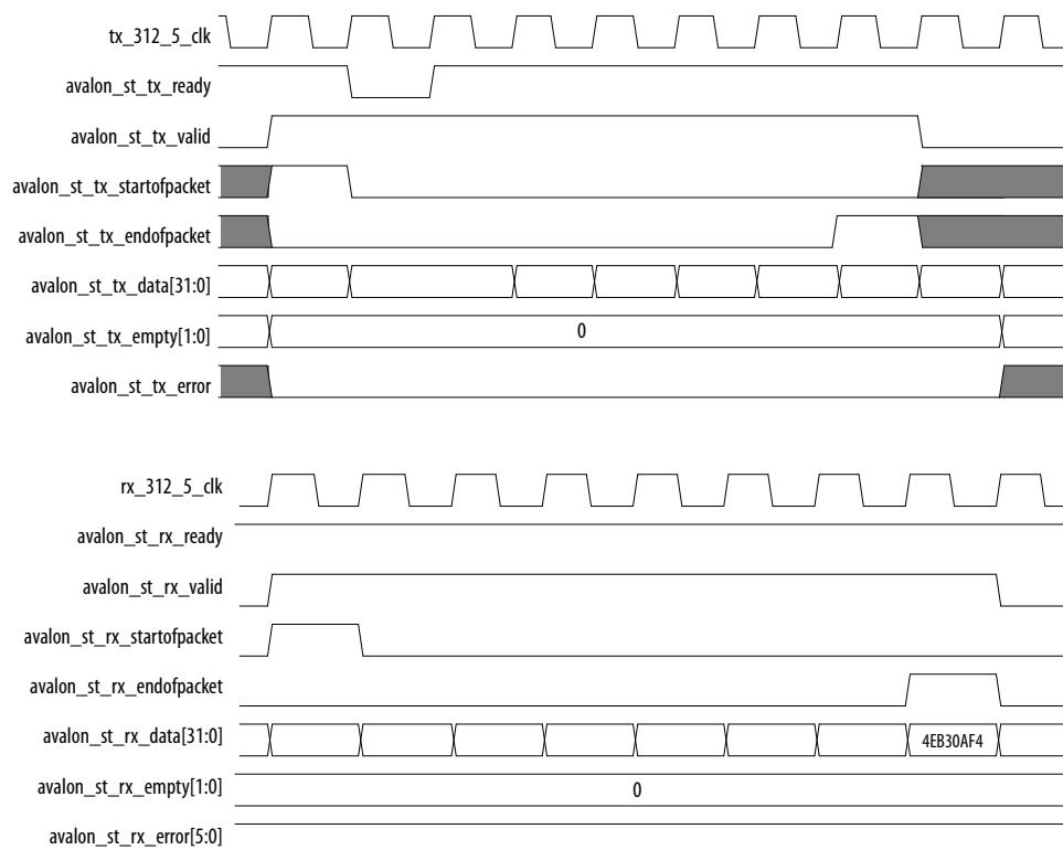
Figure 11. Avalon Streaming TX and RX Interfaces with CRC Insertion Enabled
