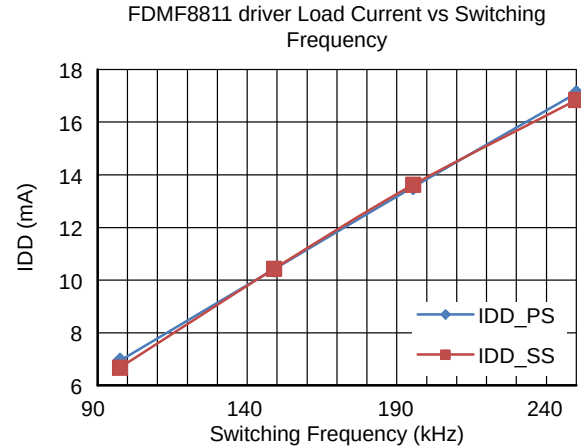
Figure 20. Driver Current per FDMF8811 vs. Switching Frequency
