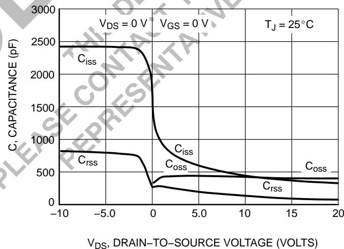
Figure 7. Capacitance Variation
