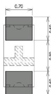
Figure 1. IN-S63FTHIR Solder Pattern
