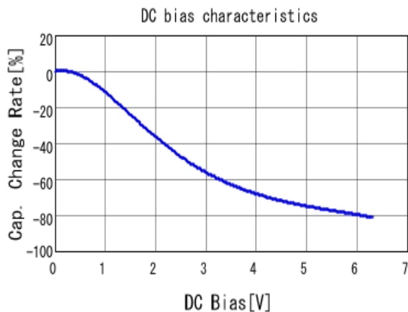
■ GRM31CR60J227ME11 C-DC bias capchange, 25.0degC, AC0.
