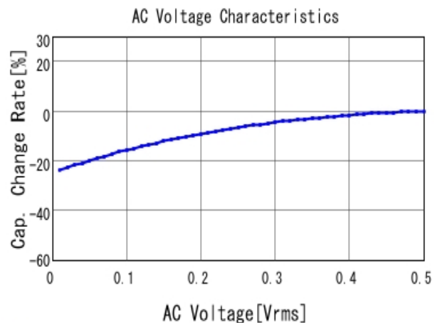
■ GRM31CR60J227ME11 C-AC Voltage capchange, DC0V, 25.0d
