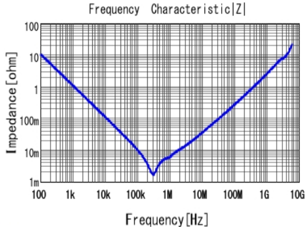
■ GRM31CR60J227ME11 |Z| DC0V, 25degC
