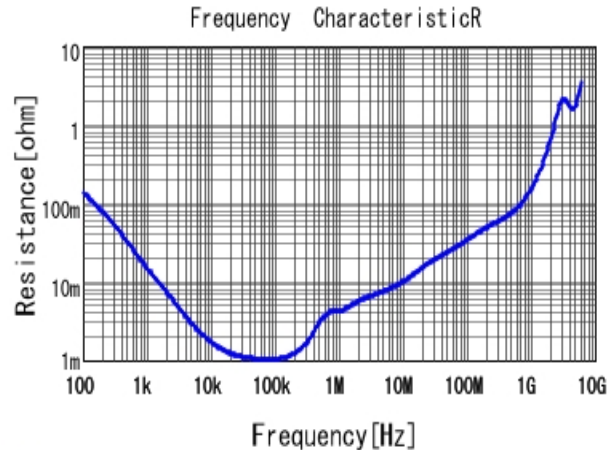
■ GRM31CR60J227ME11 R DC0V, 25degC
