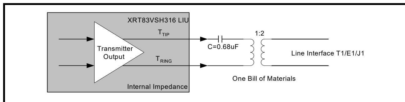
FIGURE 23. TYPICAL CONNECTION DIAGRAM USING INTERNAL TERMINATION
