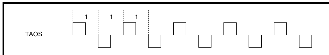
FIGURE 20. TAOS (TRANSMIT ALL ONES)
