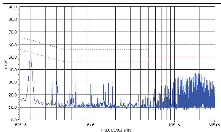
Graph 1. Conducted emissions performance, Positive Line, CISPR 22, Class B, 48 Vin, full load
