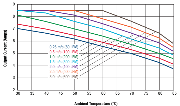
Maximum Current Temperature Derating at sea level ( V_{in}=48V , longitudinal airflow, on 10'' \times 10'' PCB with baseplate)
