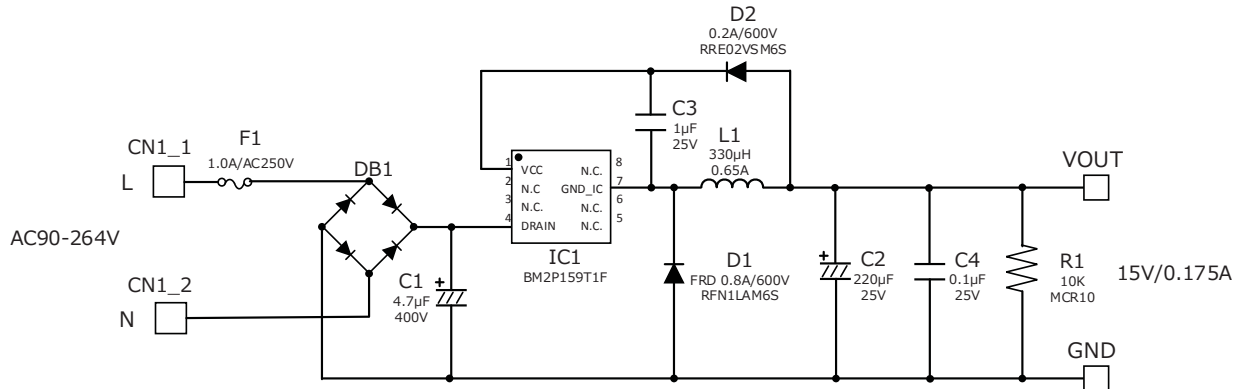
Figure 23. BM2P159T1F-EVK-001 Schematics
