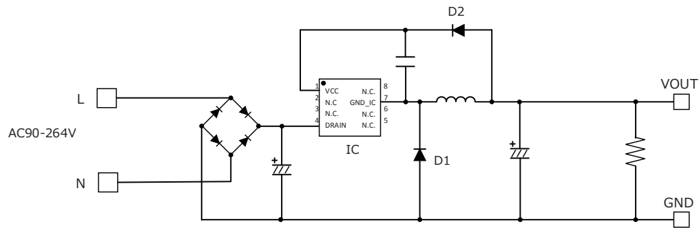
Figure 4. BM2P159T1F-EVK-001 Application Circuit
