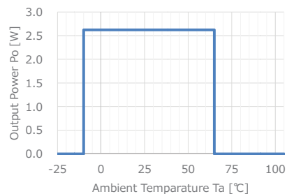
Figure 3. Temperature Derating curve
