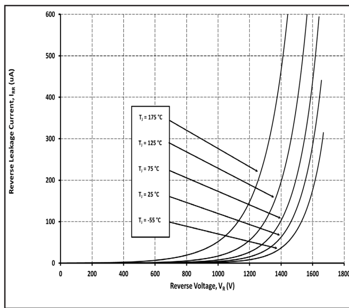
Figure 2. Reverse Characteristics
