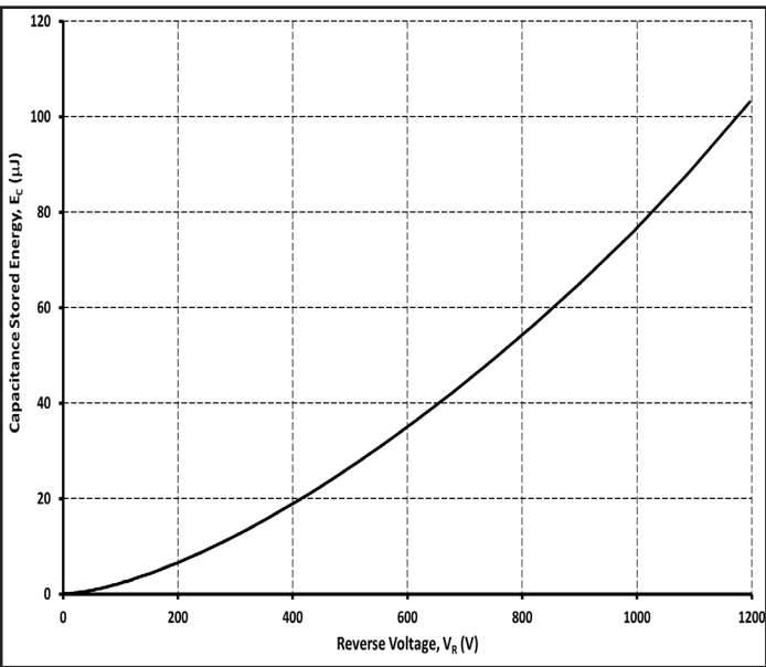
Figure 7. Typical Capacitance Stored Energy
