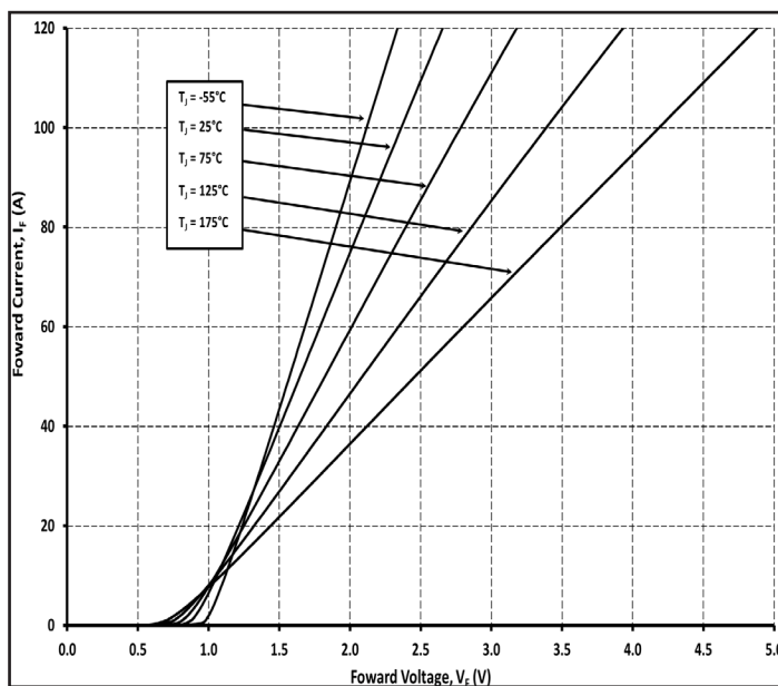
Figure 1. Forward Characteristics
