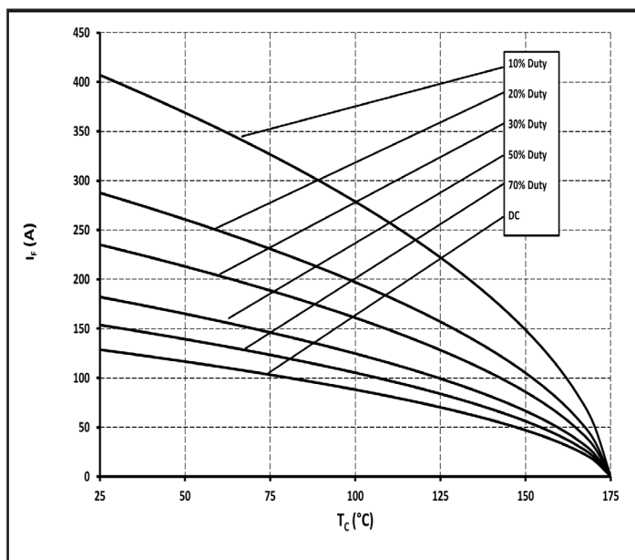
Figure 3. Current Derating
