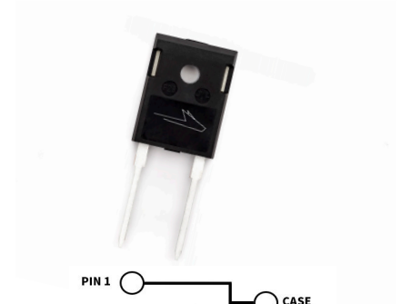
Package Types: TO-247-2 Marking: C4D40120H
