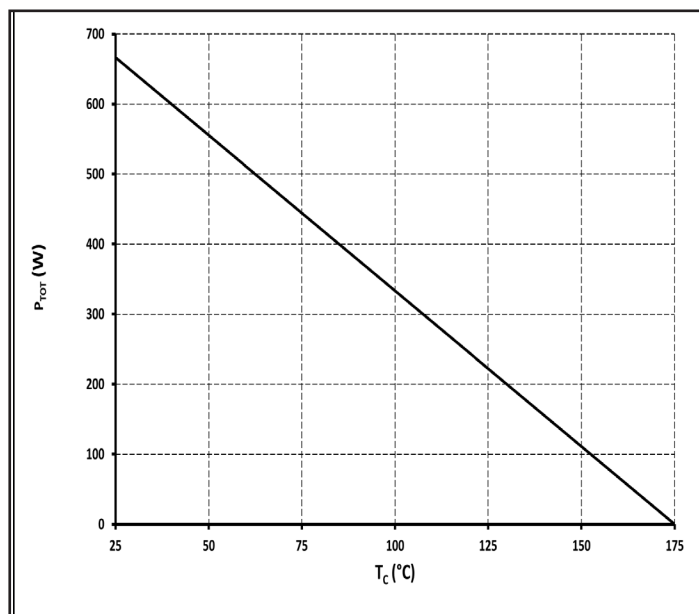
Figure 4. Power Derating
