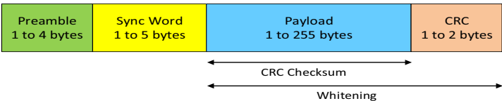
Figure 7-2: Fixed-length Packet Format
