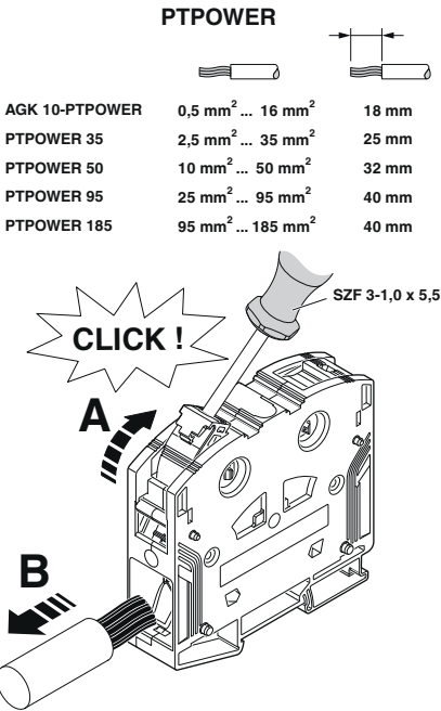
Schematic diagram
