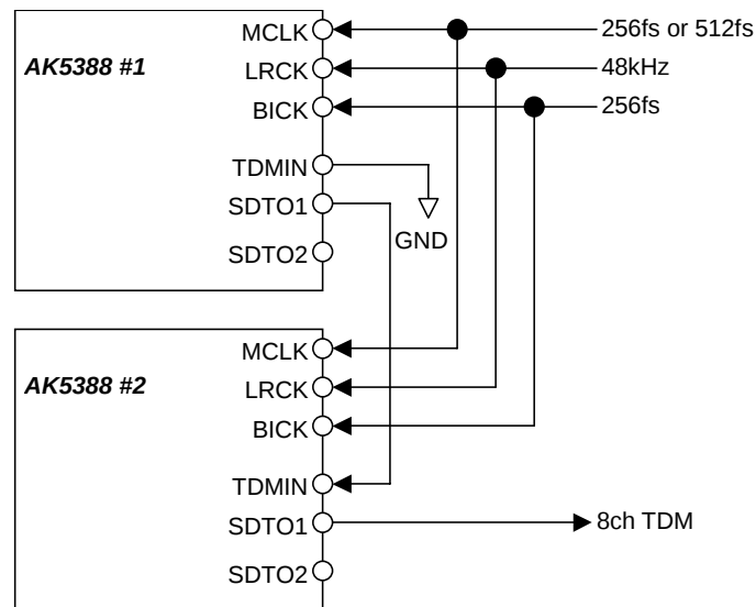
Figure 17. Cascade TDM Connection Diagram
