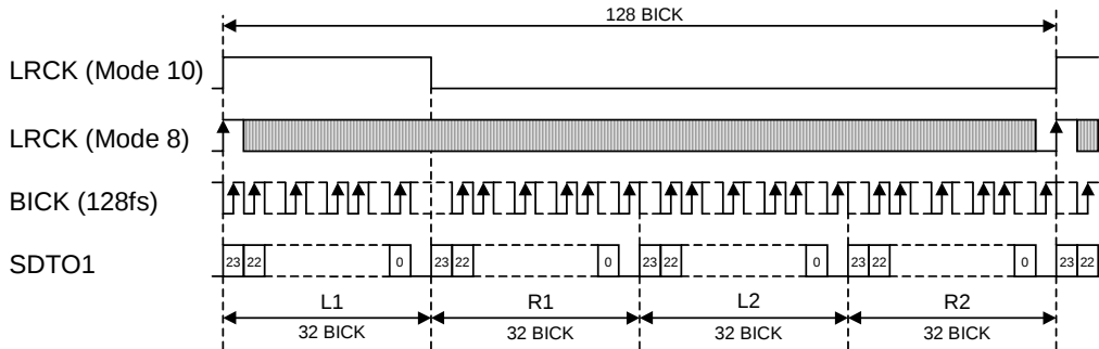
Figure 14. Mode 8/10 Timing (TDM128 mode, MSB justified)
