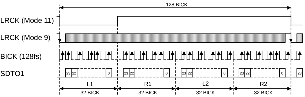
Figure 15. Mode 9/11 Timing (TDM128 mode, I 2 S Compatible)
