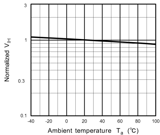
Fig. 12.10 Normalized V_H - T_a
