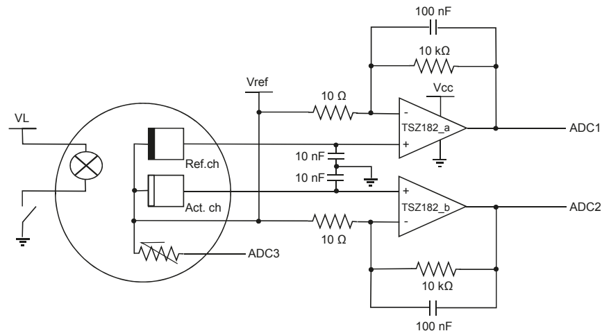
Figure 62. Principle schematic
