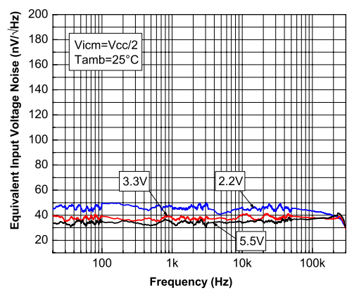
Figure 29. Noise vs. frequency
