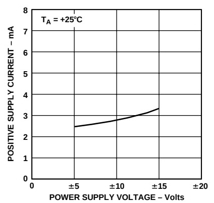
Figure 25. Positive Supply Current vs. Supply Voltage
