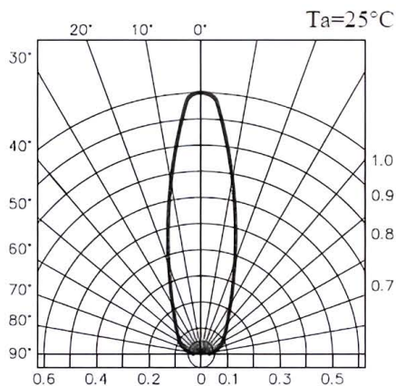
Radiation Diagram
