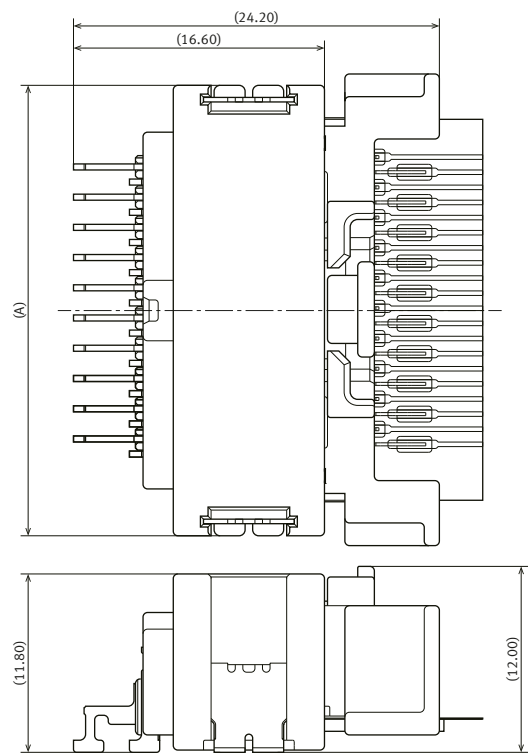
External dimensions
