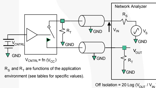
Figure 17. Channel Off Isolation
