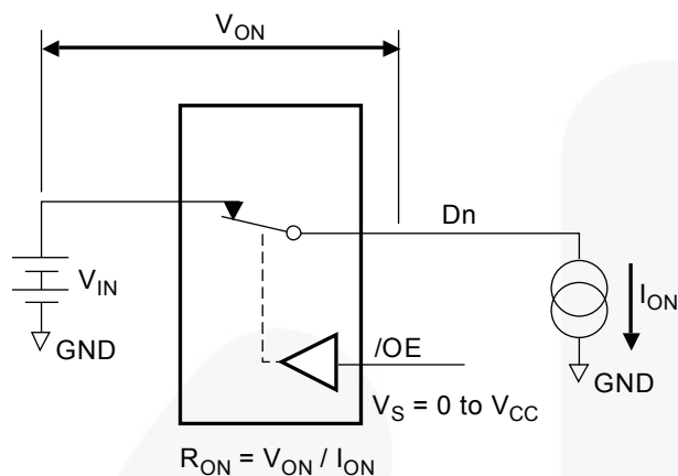
Figure 8. On Resistance
