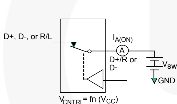
Figure 10. On Leakage
