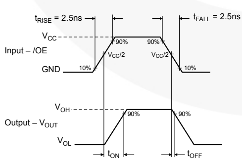
Figure 12. Turn-On / Turn-Off Waveforms
