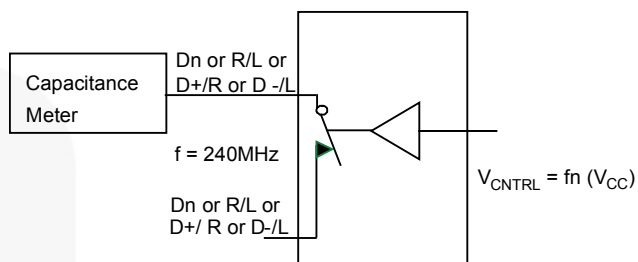
Figure 15. Channel On Capacitance
