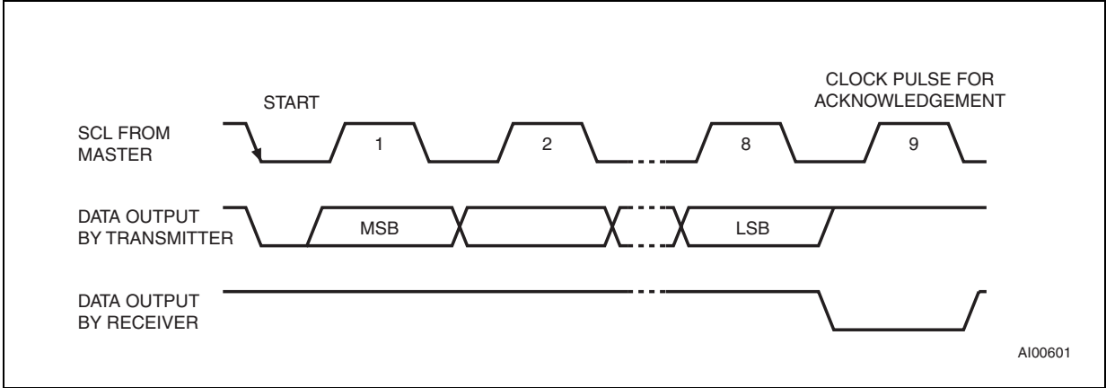
Figure 5. Acknowledgement sequence
