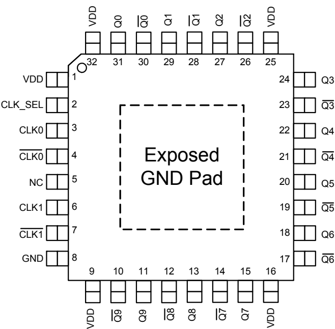
Figure 12. 32-eLQFP Pin Diagram (Top View)
