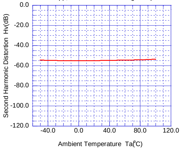
Second Harmonic Distortion vs. Temperature
