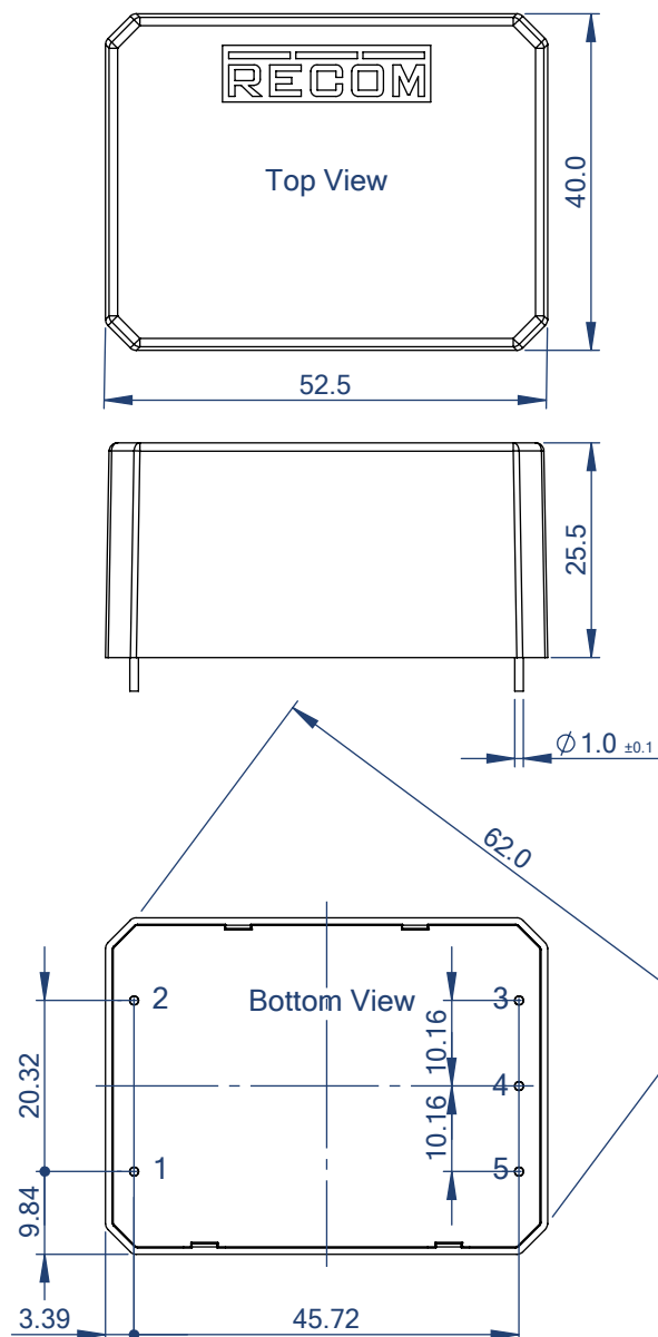
Dimension Drawing “/277/HT” Version (mm)
