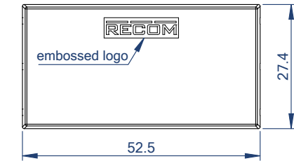
Dimension Drawing “/277” & “/277/CC” (mm)
