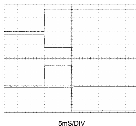
Figure 14. T_{\text{BLANK}} Response ( V_{\text{DRV}} signal forces the device to go into overcurrent condition.)
