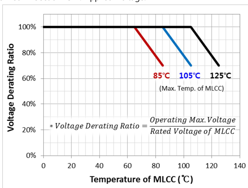
Derating A
